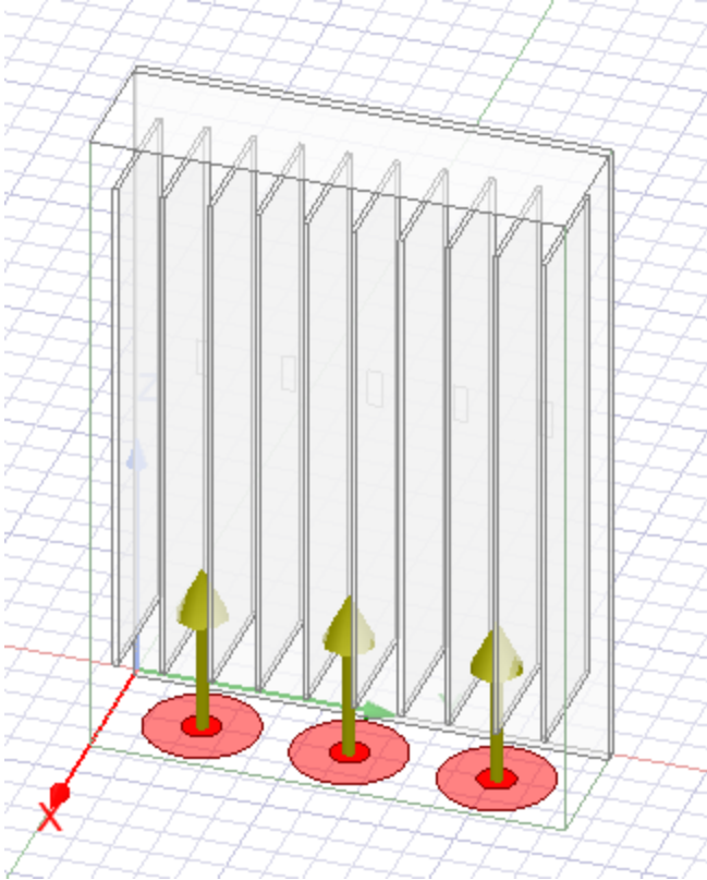
Figure 1-1: Finned Heat Sink
